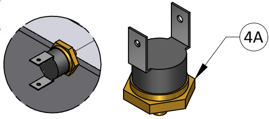
DETAIL A
